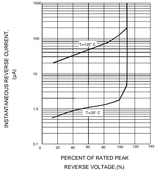
FIG.4-TYPICAL REVERSE CHARACTERISTICS
